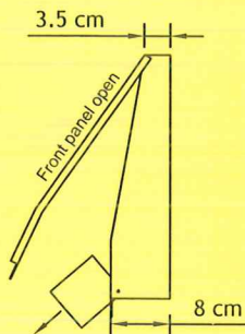
Side view showing the internal cigarette collection tray in emptying mode
